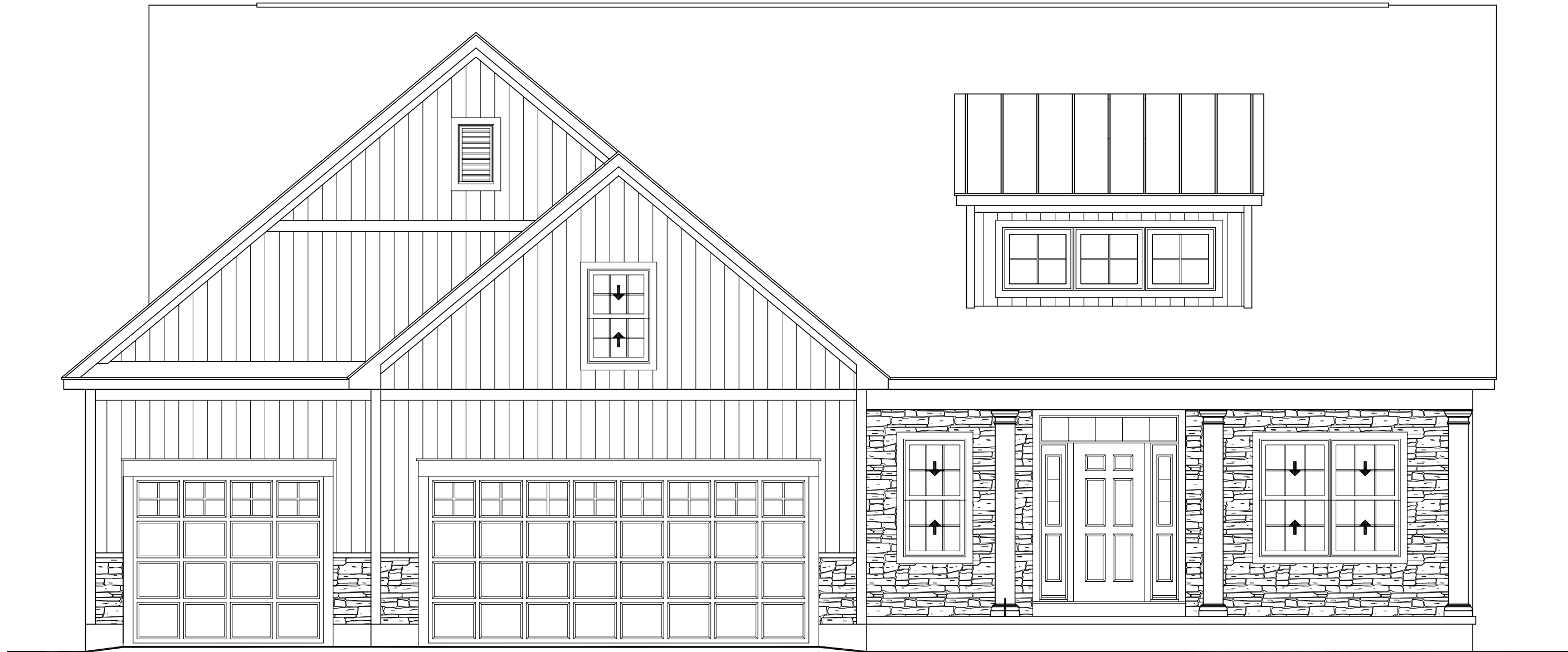
FRONT ELEVATION
